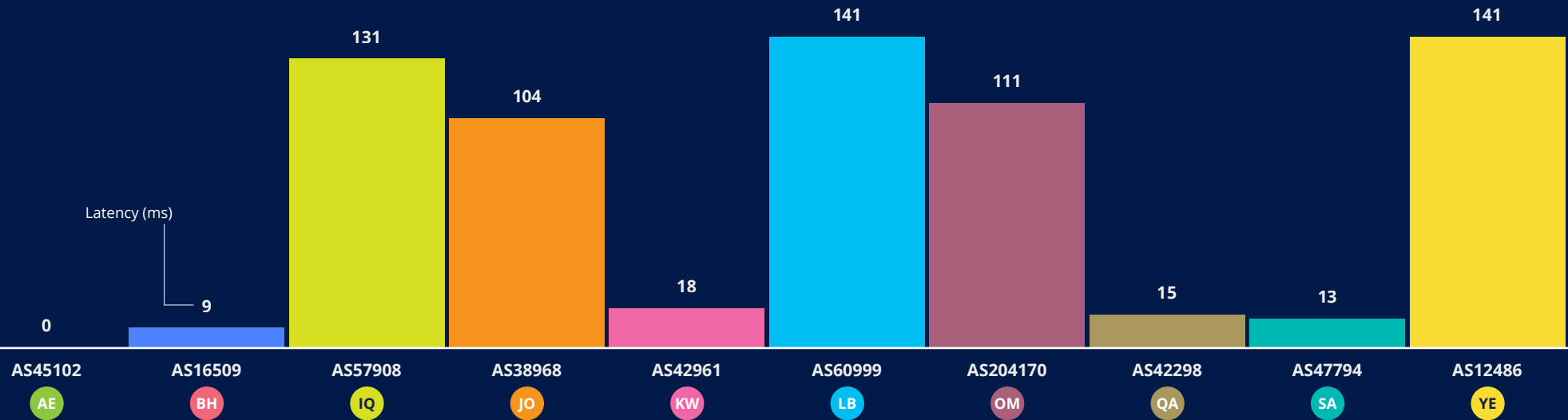
Figure 10: Reaching a regional streaming platform in UAE-IX using an IPv4 destination
